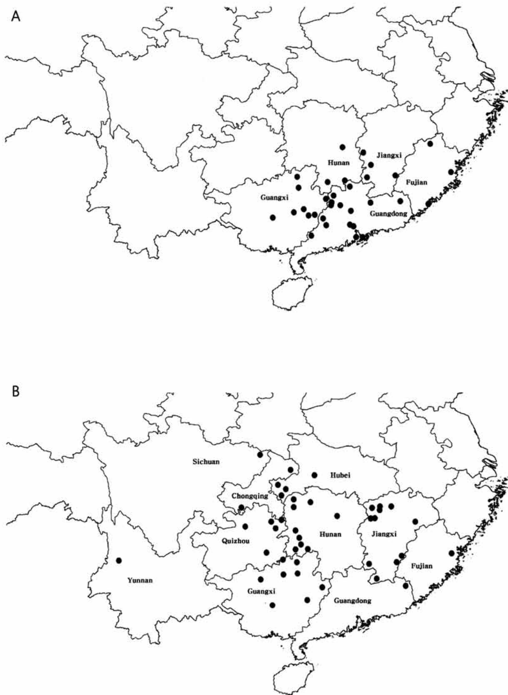
Fig. 5. Distribution maps of Acer wilsonii (A) and A. tutcheri (B) in southern China.
